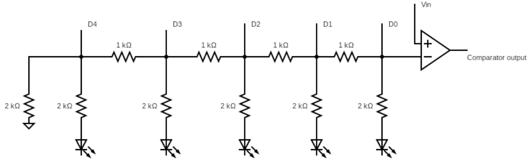
Figure 5: DAC circuit
